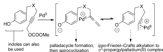
Scheme 1. Reaction design.
