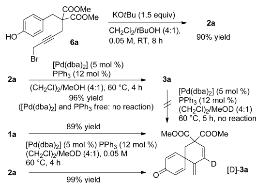
Scheme 3. Experiments for elucidating the reaction mechanism.
